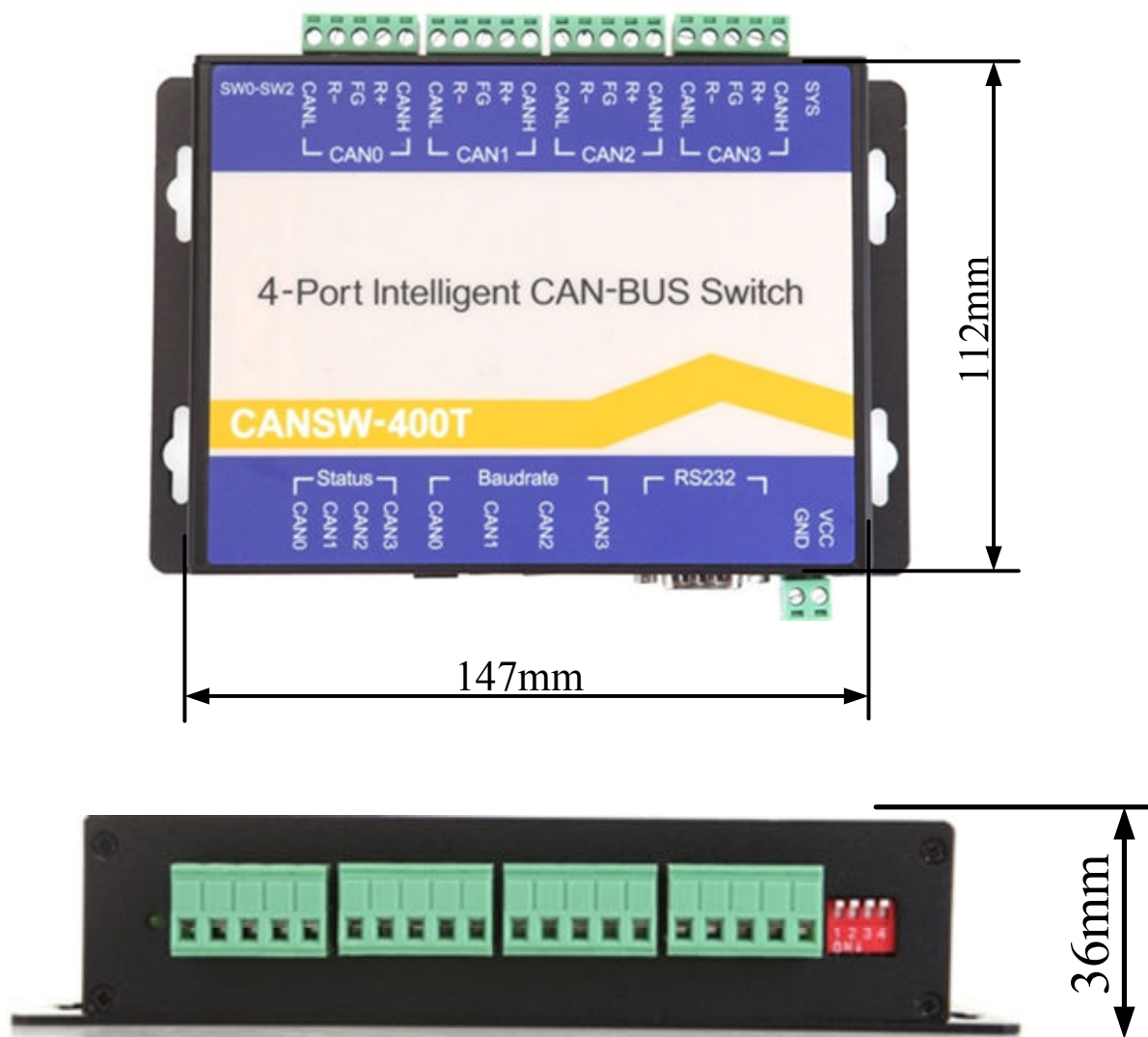
Figure 2-1-1 SW-400T
