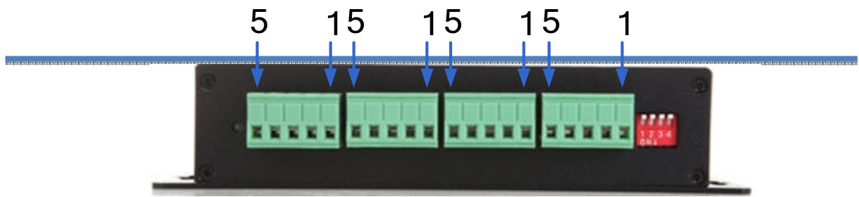
Figure 2-2-2-1 CAN Terminals
