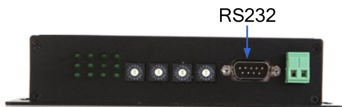
Figure 2-2-6-1 RS232 port
