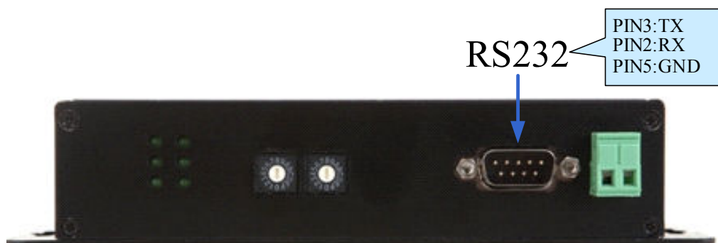
Figure 2-2-6-1 RS232 Interface
