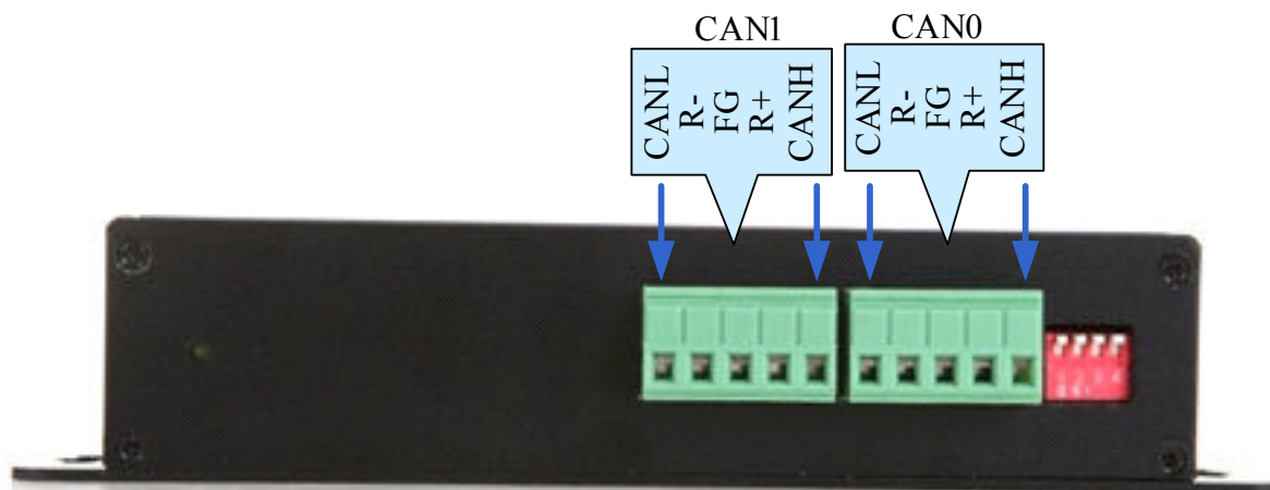
Figure 2-2-2-1 CAN Interface
