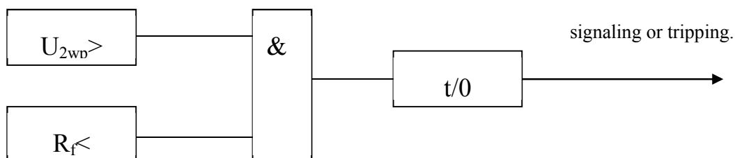
Figure 5-9 Tripping logic of generator rotator two-points ground protection
