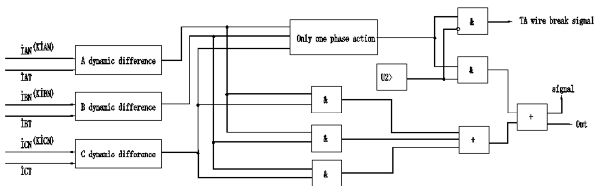
Figure 5-2 Cyclic lockout mode generator differential protection logic diagram
