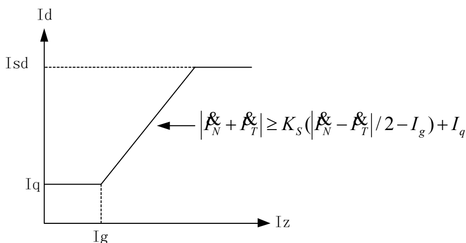
Figure 5-1 Ratio braking characteristic curve
